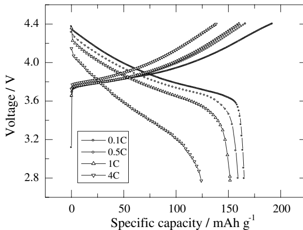
Fig. 6. Charge/discharge curves of Li/Li[Ni 1/2 Mn 1/2 ]O 2 cells at various current densities between 2.8 and 4.4 V. Each cell was charged using a current density of 0.32 mA cm -2 (0.2 C rate) and discharged using various current densities.
