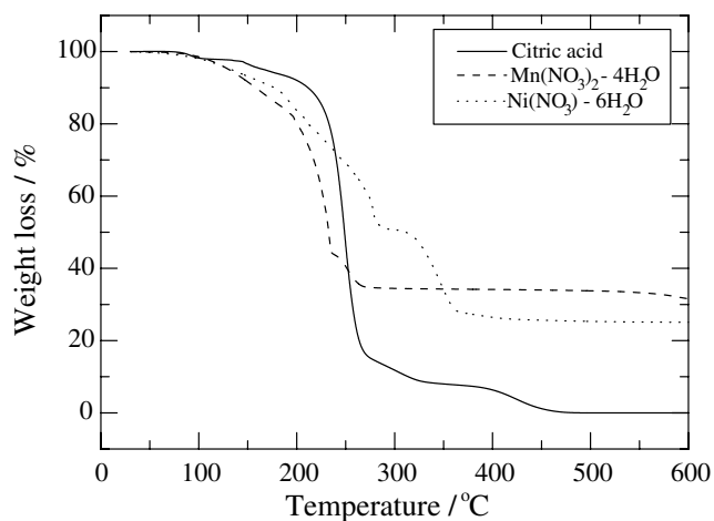
Fig. 1. Thermogravimetric analysis of the starting materials. The mixture was dried in a vacuum oven at 25 °C prior to the thermal analysis and the heating rate was 5 °C \text{min}^{-1} in air.
